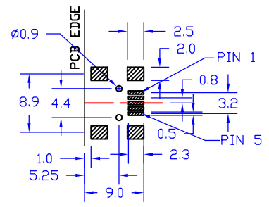
PCB Layout (Top View) (Scale 2:1)
